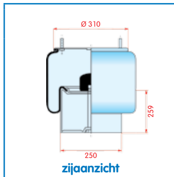
Luchtbalg compleet (Complete Assembly) Type 3670 S
