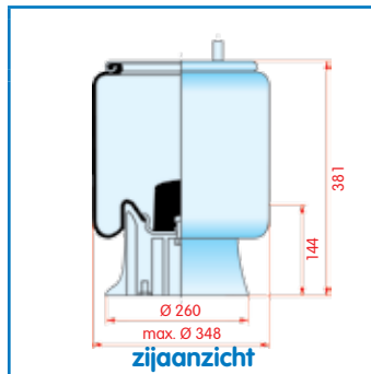
Luchtbalg compleet (Complete Assembly)
